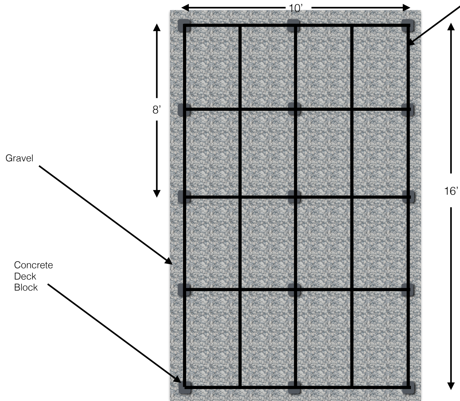
Deck Base Plan View
